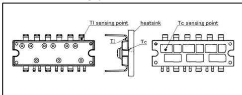
Tc, Tl sensing point
