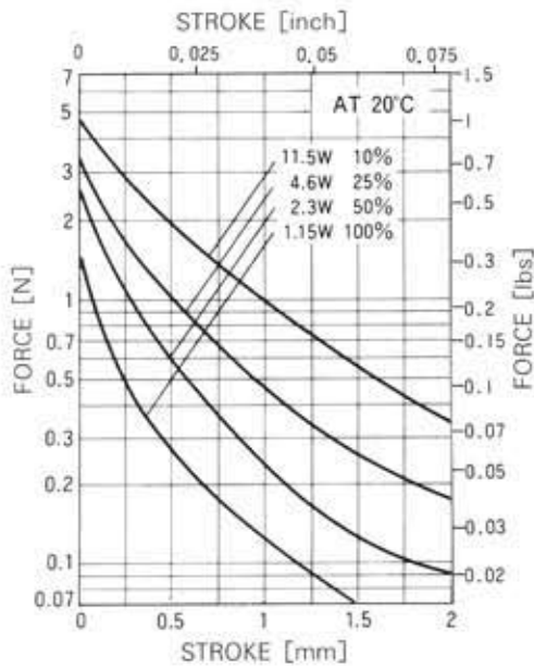
STROKE - FORCE
