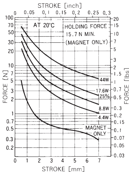
STROKE - FORCE
